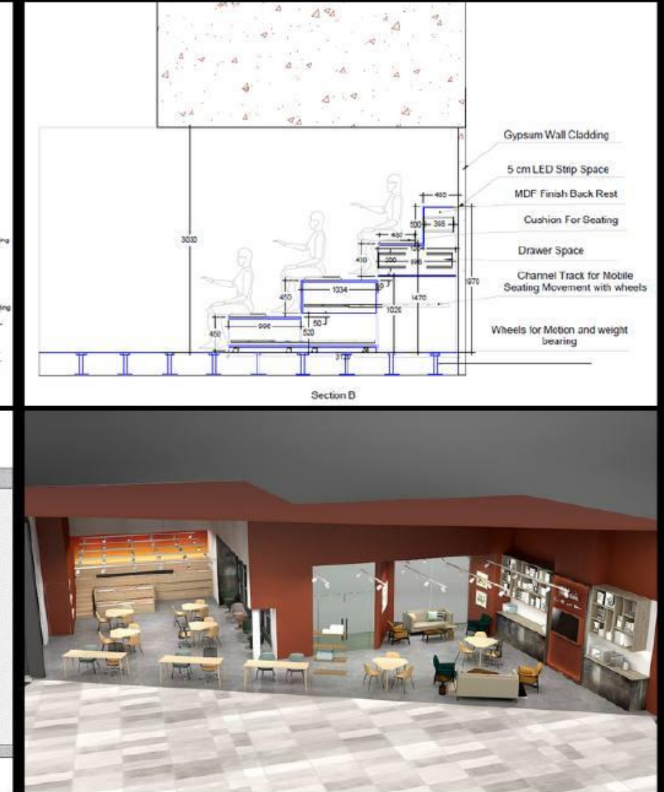
DETAILED DRAWING
