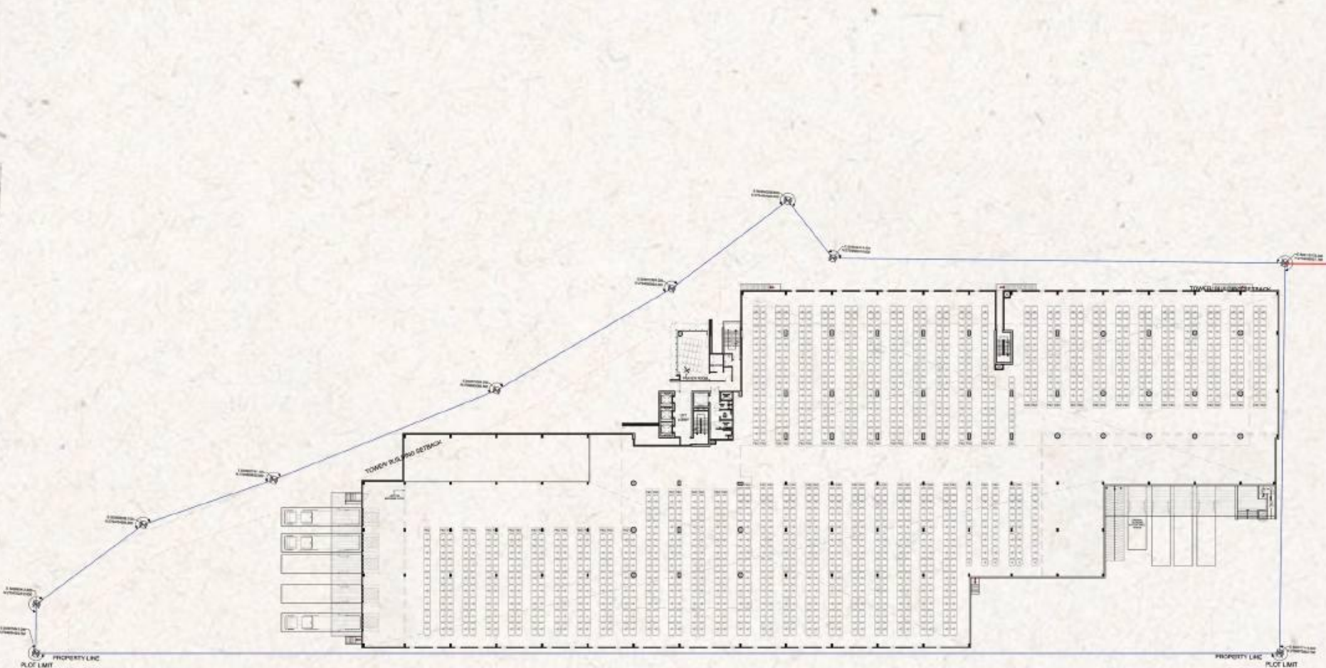
MAZZANINE FLOOR PLAN
