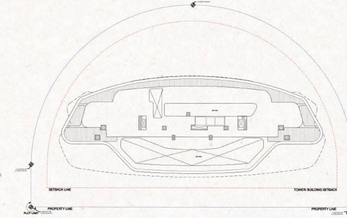
ROOF FLOOR PLAN
