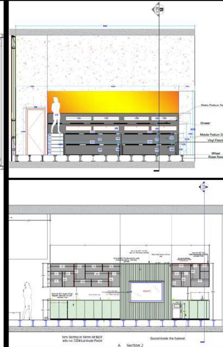
DETAILED DRAWING
