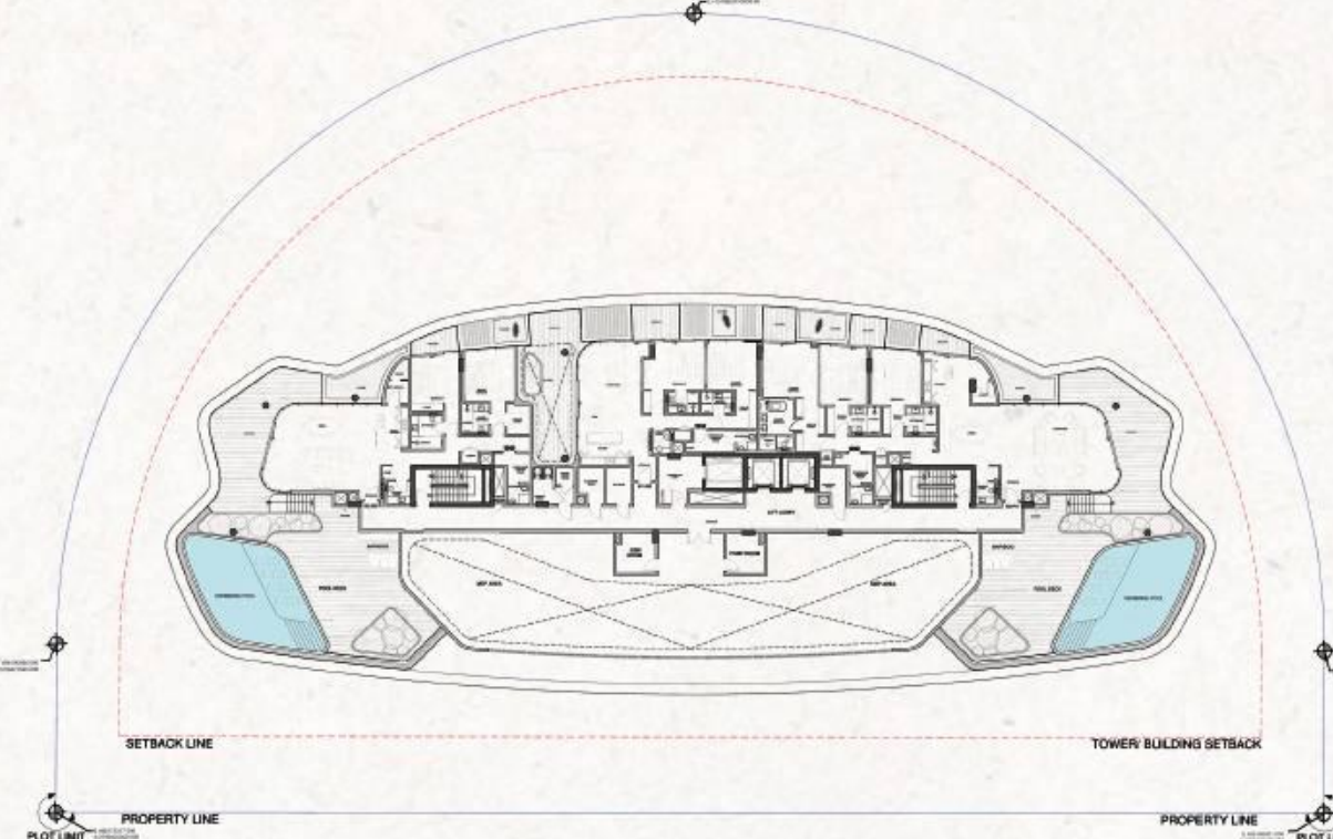
EIGHTH FLOOR PLAN
